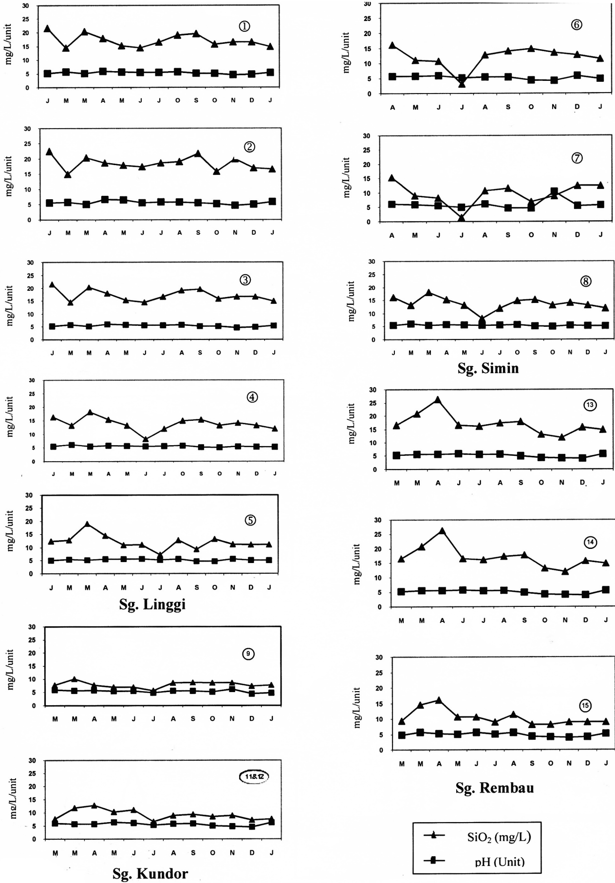
FIGURE 2. Monthly variation in silica (SiO 2 ) and pH at 15 main station in the Linggi River Basin
