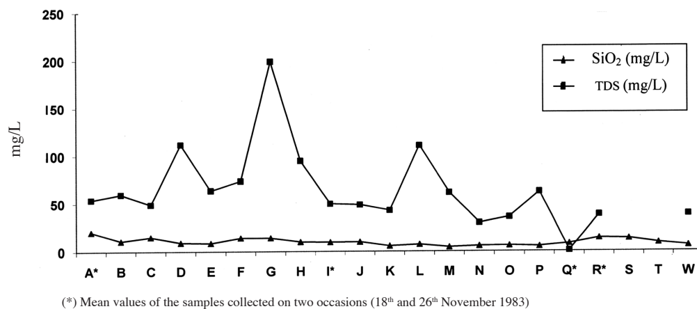
FIGURE 5. Silicate (SiO 2 ) and total dissolved solid (TDS) at various tributaries in the Linggi River Basin
