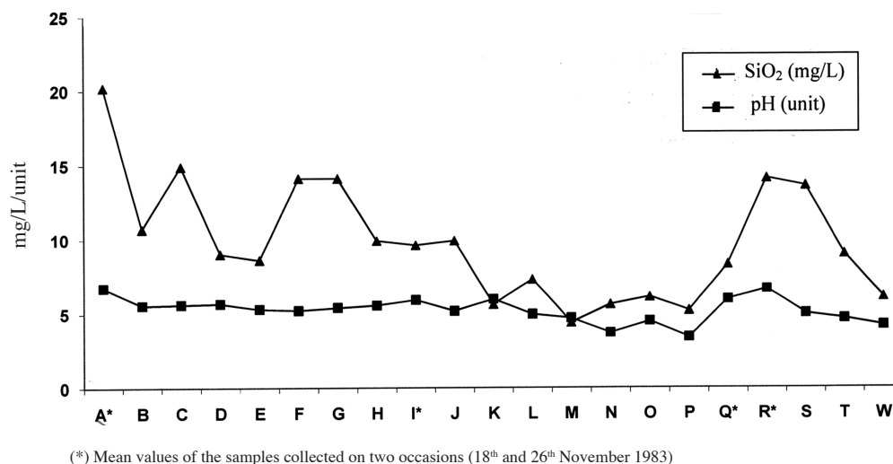
FIGURE 4. Silicate (SiO 2 ) and pH at various tributaries in the Linggi River Basin
